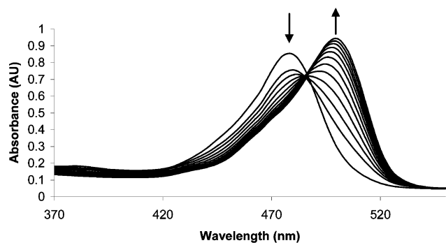
Figure 3. UV-vis spectra of 1 ( 4 \times 10^{-6} M) and L-cysteine ( 4.9 \times 10^{-5} – 7.4 \times 10^{-4} M) in deproteinized human plasma at room temperature containing 1.0 mM added glutathione (pH 9.5). Each spectrum is acquired 5 min after cysteine addition. As the concentration of L-cysteine increases, a red shift from 480 to 500 nm is observed.
